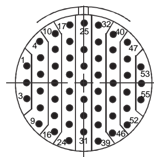
E35, Shell Size 17 55 Contacts
